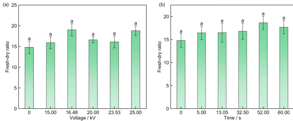
图5 电压、时间对鲜干比的影响 Fig.5 Effects of voltage and time on the ratio of fresh to dry
