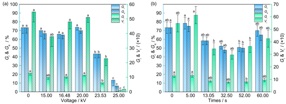
图3 电压、时间对发芽指标的影响 Fig. 3 Effect of voltage and time on germination index
