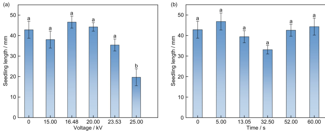
图4 电压、时间对苗长的影响 Fig. 4 Effects of voltage and time on seedling length
