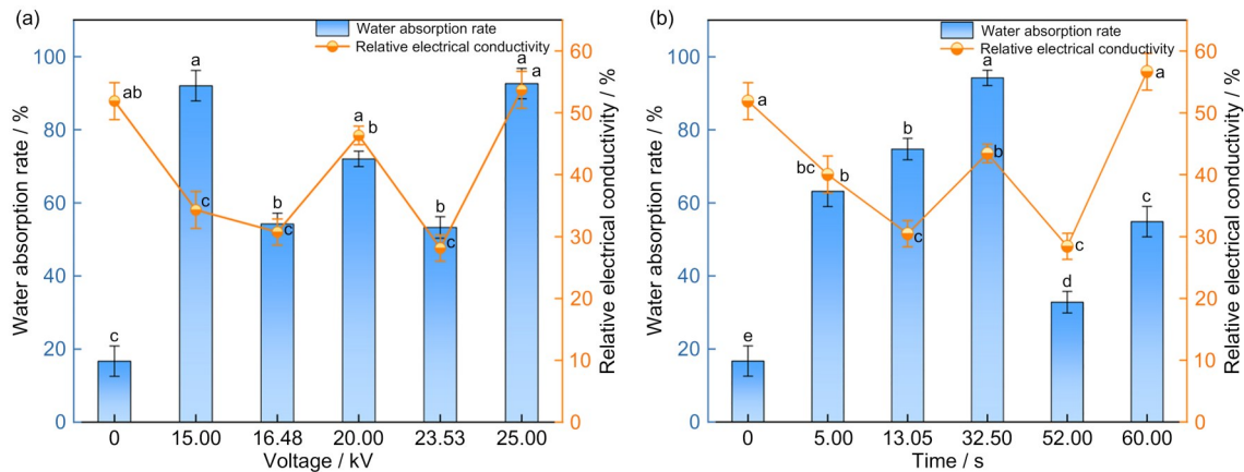
图6 电压、时间对吸水率和相对电导率的影响 Fig.6 Effects of voltage and time on water absorption and relative conductivity
