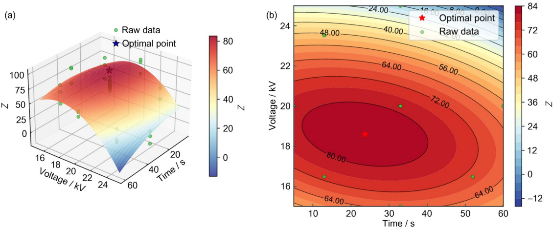
图8 二因素对苜蓿综合发芽实验指数的响应面和等高线图 Fig.8 Response surface and contour map of two factors on comprehensive germination index of alfalfa
