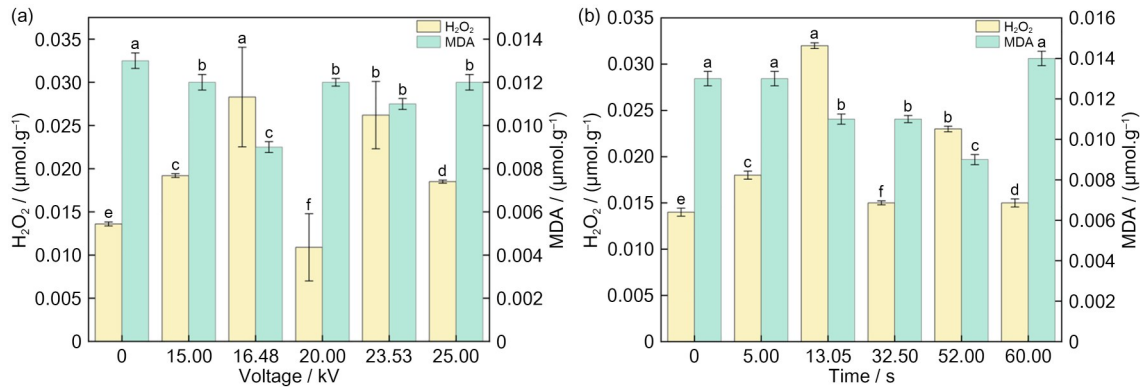
图7 电压、时间对种子H 2 O 2 和MDA的影响 Fig.7 Effects of voltage and time on seed H 2 O 2 and MDA
