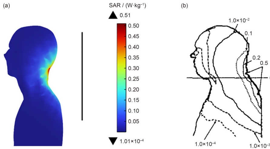
图7 人体表面SAR分布：(a)本文计算结果；(b)文献中结果 Fig. 7 Surface distribution of human body SAR: (a) the results in this paper; (b) the results in the reference
