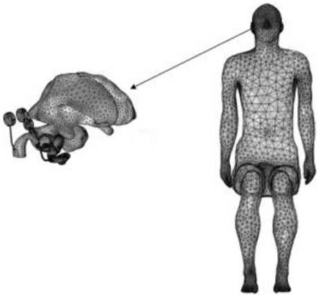
图6 佩戴人工耳蜗乘客的网格剖分 Fig. 6 Mesh grids of passengers with cochlear implants
