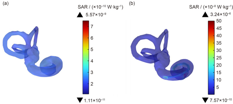
图10 内耳SAR分布:(a)普通乘客;(b)佩戴人工耳蜗乘客 Fig.10 Distribution of SAR within the inner ear: (a) ordinary passengers; (b) passengers with cochlear implants
