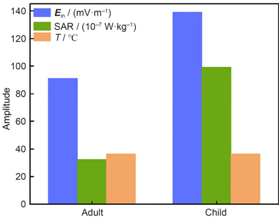
图12 不同年龄乘客内耳暴露水平对比 Fig. 12 Comparison of inner ear exposure levels for passengers with different ages
