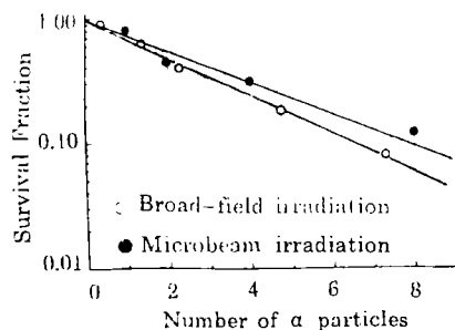
Fig.5 Comparison of the survival fraction of A_L cells either traversed with an exact number of \alpha particles through the nuclei (microbeam irradiation) or from the data obtained using average \alpha particle traversals (broad-field irradiation)
