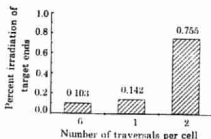
Fig.4 The probability of hitting the cell cytoplasm with the desired number of \alpha particles was 75.5%, 14.2% probability for hitting the target cytoplasm with half the desired number of particles, and 10.3% probability of not hitting the cytoplasm
