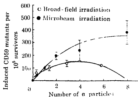
Fig.6 Comparison of the mutation induction at the CD59^- locus of A_L cells irradiated with an exact number of \alpha particles through the nuclei (microbeam irradiation) or from the data obtained using average \alpha particle traversals (broad-field irradiation)
