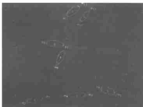
Fig.3 Fluorescent imaging of A_L cells stained with Hoechst 33342 for nucleus and Nile Red for cytoplasm and viewed by the image analysis system under a 40X objective lens
